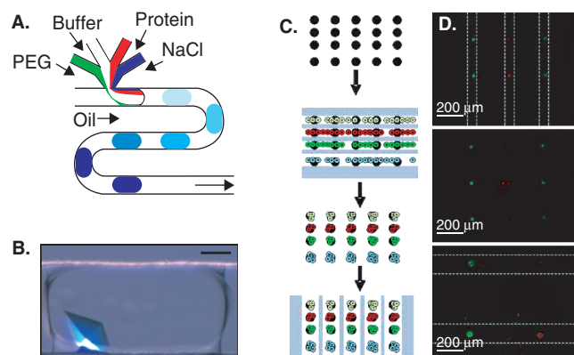
Figure 4. Microfluidic approaches for protein crystallization and cell-based screening. A. Multiphase fluids can be used to generate droplets inside microchannels comprised of proteins, precipitants and additives. B. A protein crystal (thaumatin) inside a droplet within a microfluidic device. Scale bar is 50 µm. (Reprinted with permission from ZHENG et al. : Copyright (2003), American Chemical Society) [101]. C. Schematic image of the formation of multiphenotype cell arrays within microchannels containing microwells. A reversibly-sealed microfluidic device was aligned on top of a microwell array to control the delivery of liquid to each well. D. Fluorescent images of scheme C . Cells were labeled with membrane dyes (CFSE, green) and SYTO (red). Different cell types (ESCs, AML12, and NIH 3T3 cells) are shown in the image (KHADEMHOSSEINI et al. : Lab. Chip 5 :1380-1386 [21]). Reproduced by permission of The Royal Society of Chemistry).
