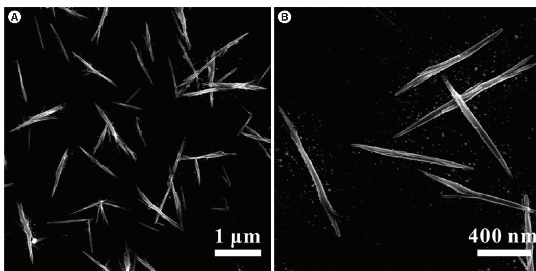
Figure 2. Scanning electron microscope micrographs of mobile nanoneedles carrying two drugs. Reproduced with permission from [25], licensed with CC BY 4.0.
