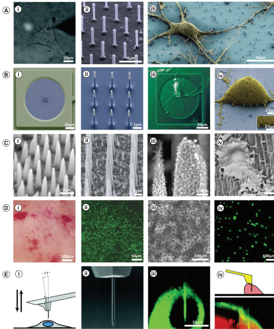
Figure 5. Applications of nanoneedle-like structures. (A) Intracellular delivery of fluorescent quantum dots into HeLa cells: (i) Micrograph of nanoneedle penetrating a HeLa cell, (ii) SEM micrograph of vertical silicon nanowires fabricated using etching, (iii) SEM micrograph of rat hippocampal neuron seeded on etched silicon nanowires for plasmid DNA transfection, (B) Rat cortical neuron cultured on a vertical nanowire electrode array (VNEA) pad. (i) SEM micrograph of a VNEA pad; (ii) SEM micrograph of nine silicon nanowires on VNEA pad; (iii) DIC micrograph of a rat cortical neuron cultured on a VNEA pad and; (iv) SEM micrograph of a rat cortical neuron cultured on a VNEA pad, (C) (i–iii) SEM micrograph of Cy3-labelled GAPDH-siRNA and GFP-expressing DNA plasmid retaining porous silicon nanoneedles developed to transfect HeLa cells and; (iv) SEM micrograph of HeLa cells seeded over nanoneedles. (D) Nano-injected mice muscle exhibiting greatest (i) vascularization using intravital bright-field and; (ii) hVEGF165 expression using confocal microscopy images. (iii) SEM micrograph of 15.14% TiCu nanotubes and; (iv) Fluorescence image showing NO in endothelial cells. (E) Nanoneedle-incorporated atomic force microscopy cantilever system: (i) Schematic diagram of AFM nanoneedle over a cell; (ii) SEM micrograph of nanoneedle; (iii) Cross-section confocal micrographs of nanoneedle successfully penetrating a HEK293 cell and; (iv) Reconstructed 3D image from confocal slices of AFM nanoneedle penetrating HEK293 cell.
